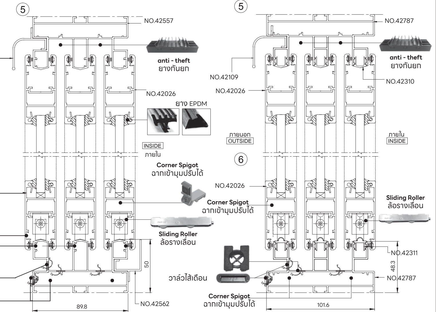
SECTION-B VERTICAL SECTION DETAIL FRAME WIDTH 100 mm.
