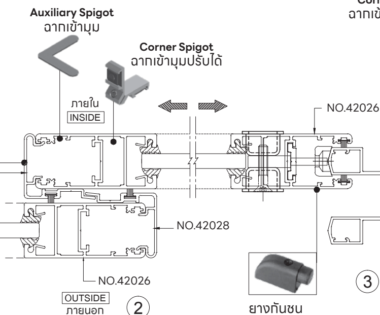
SECTION-B VERTICAL SECTION DETAIL FRAME WIDTH 100 mm.
