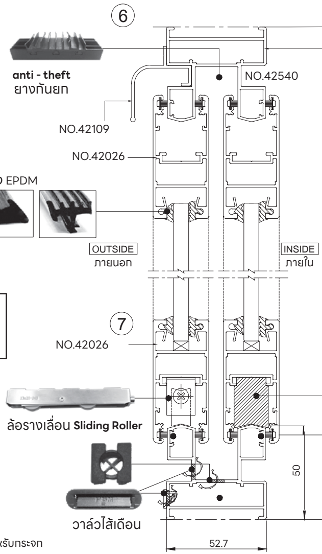
SECTION-B VERTICAL SECTION DETAIL FRAME WIDTH 50 mm.
