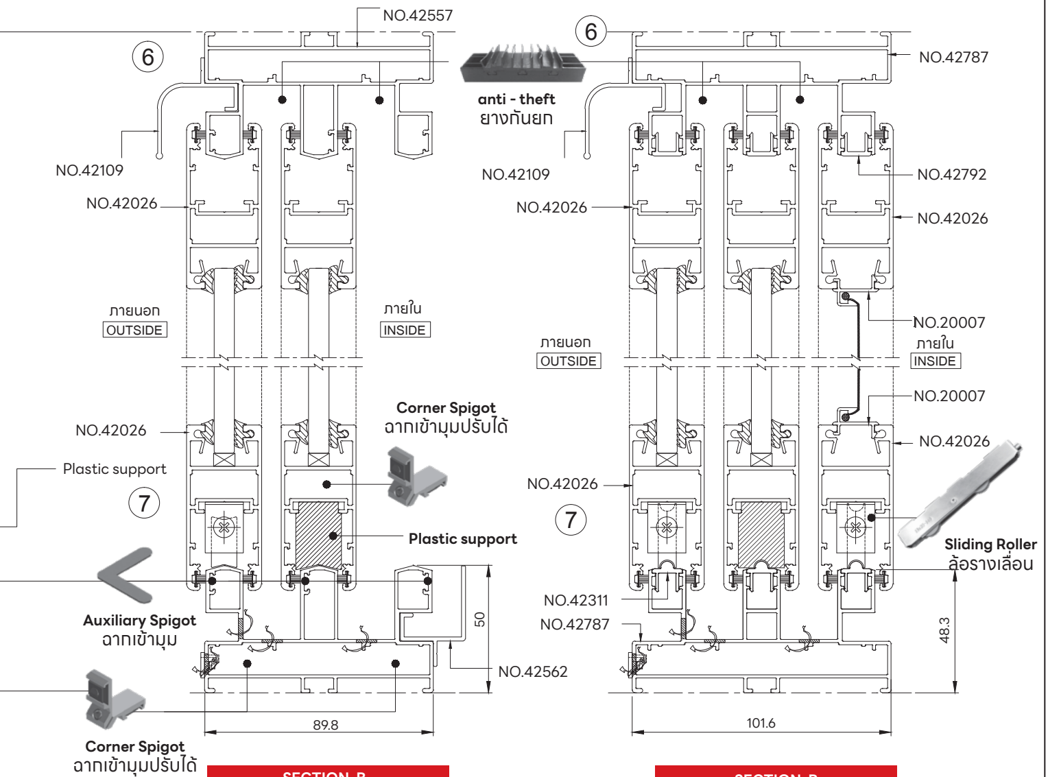
SECTION-B VERTICAL SECTION DETAIL FRAME WIDTH 100 mm.
