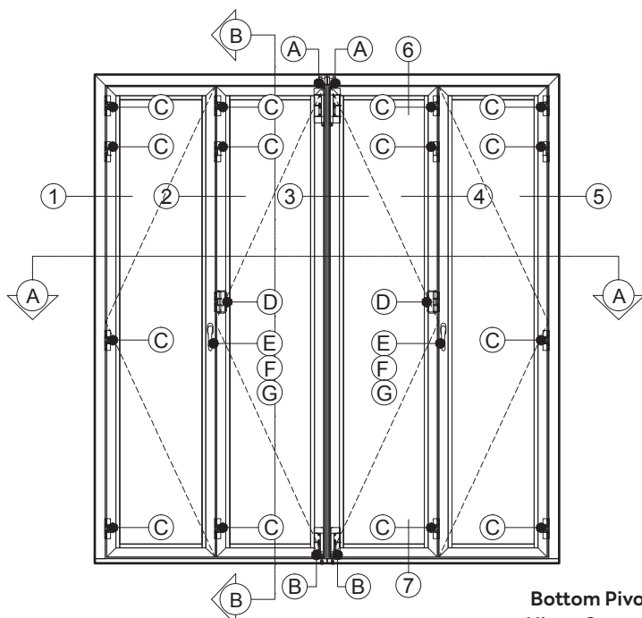
ELEVATION - 4-2-2
