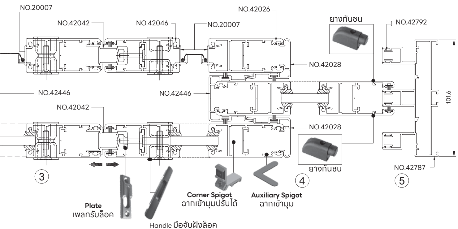
SECTION-B VERTICAL SECTION DETAIL FRAME WIDTH 100 mm.
